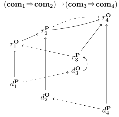
Fig. 3. A typical play for copycat
