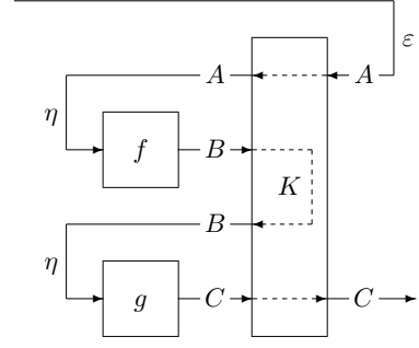
Fig. 5. Composing GAMs using the K HRAM
