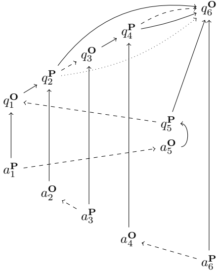
Fig. 4. Composition from copycat
