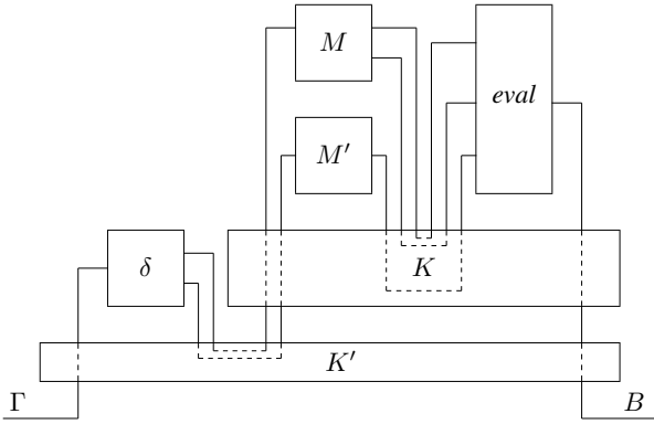
Fig. 6. GAM net for application
