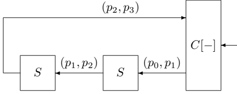
Fig. 2. Non-locality of names in HRAM composition
