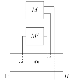
Fig. 7. Optimised GAM net for application
