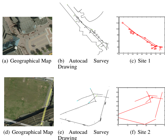
Figure 3. Geographical Map, Autocad Survey Drawing and the obtained Utility Mapping
