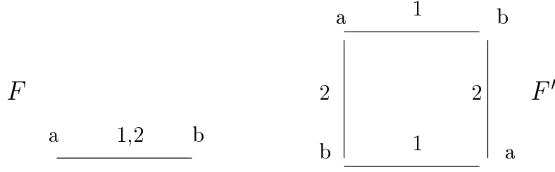
Figure 1: Two p-morphic frames used in the proof of Lemma 3.3
