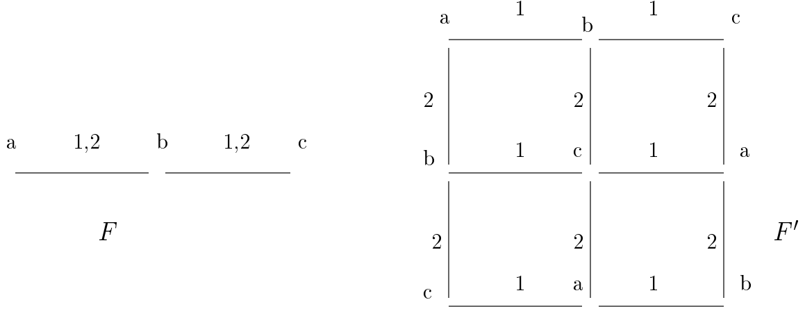
Figure 2: An EDI frame mapping an ED frame via a p-morphism
