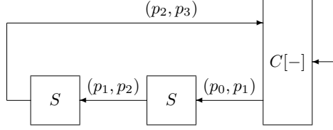
Figure 4: Non-locality of names in HRAM composition
