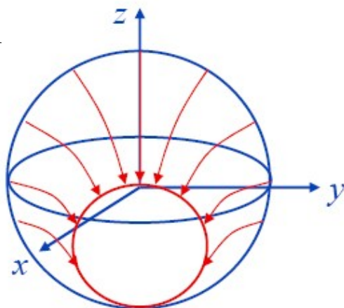
Relaxation processes
