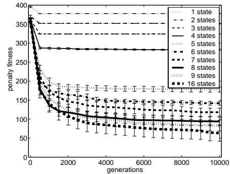
Figure 3: Fitness test experiments in the Santa Fe trail problem
