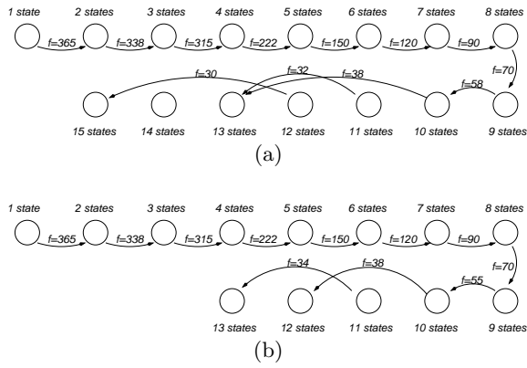
Figure 4: A partial order relation of FSMs with varying number of memory states in terms of behaviour performance (by beta distribution) (a) 50 trials (b) 25 trials (the arrow label indicates the threshold fitness for success/failure)
