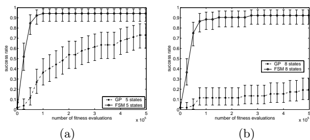
Figure 9: Run-time distribution with genetic programming and FSM controllers (the average and 95% confidence range of success rate in the beta distribution are displayed) (a) evolving five internal states (threshold fitness: 222) (b) evolving eight internal states (threshold fitness: 150)
