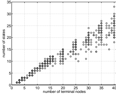
Figure 7: Relation between terminal nodes and internal states in genetic programming approach (a varying number of terminal nodes was a control parameter)
