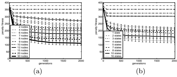
Figure 6: Genetic programming result (a) evolve controllers with a fixed number of terminal nodes (b) evolve controllers with a fixed number of states
