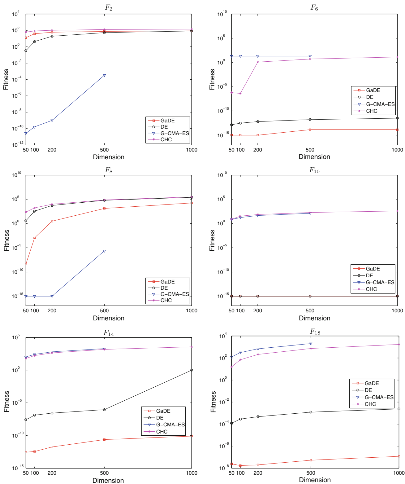
Fig. 1 The scalability curves of GaDE, DE, G-CMA-ES and real-coded CHC on functions F_2, F_6, F_8, F_{10}, F_{14} and F_{18}
