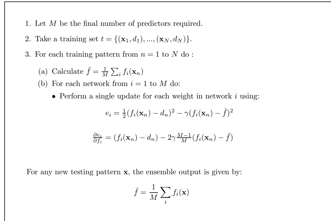
Figure 5: The Negative Correlation Learning Algorithm [33, 12]
