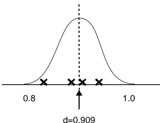
Figure 1: Typical error distribution of an unbiased estimator approximating \sin(2)
