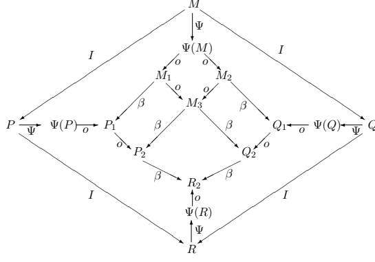
Fig. 2. The method of Ghilezan and Kunčak for the confluence of \rightarrow_I
